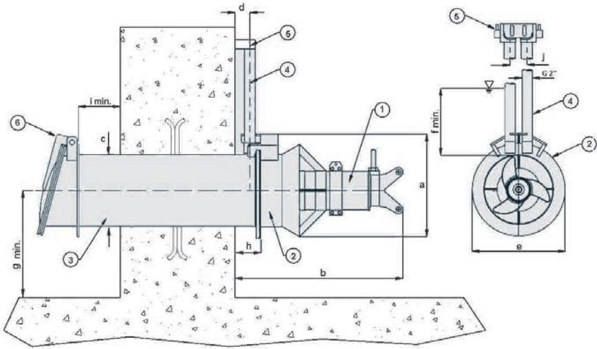
Dimensiones / Dimensions / Dimensions mm.
